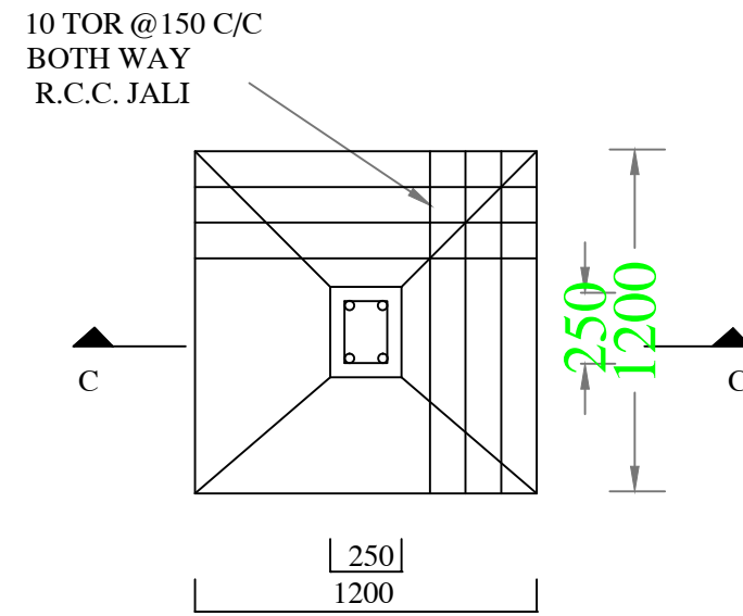
PLAN DETAIL OF FOUNDATION
