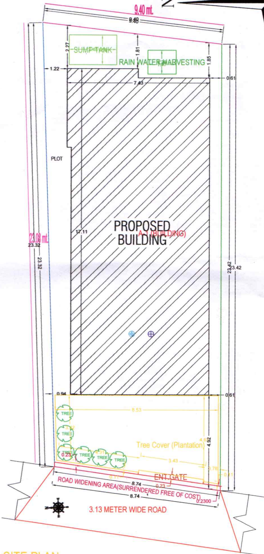
SITE PLAN
