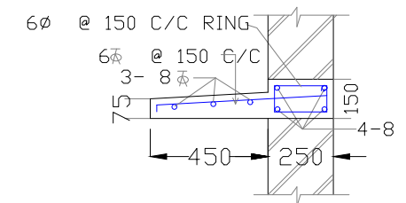
DET OF CHAJJA SCALE-1:25
