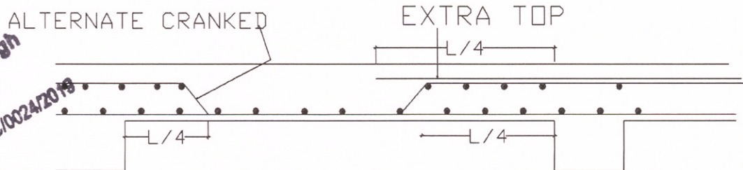
SECTION OF SLAB AT A-A'
