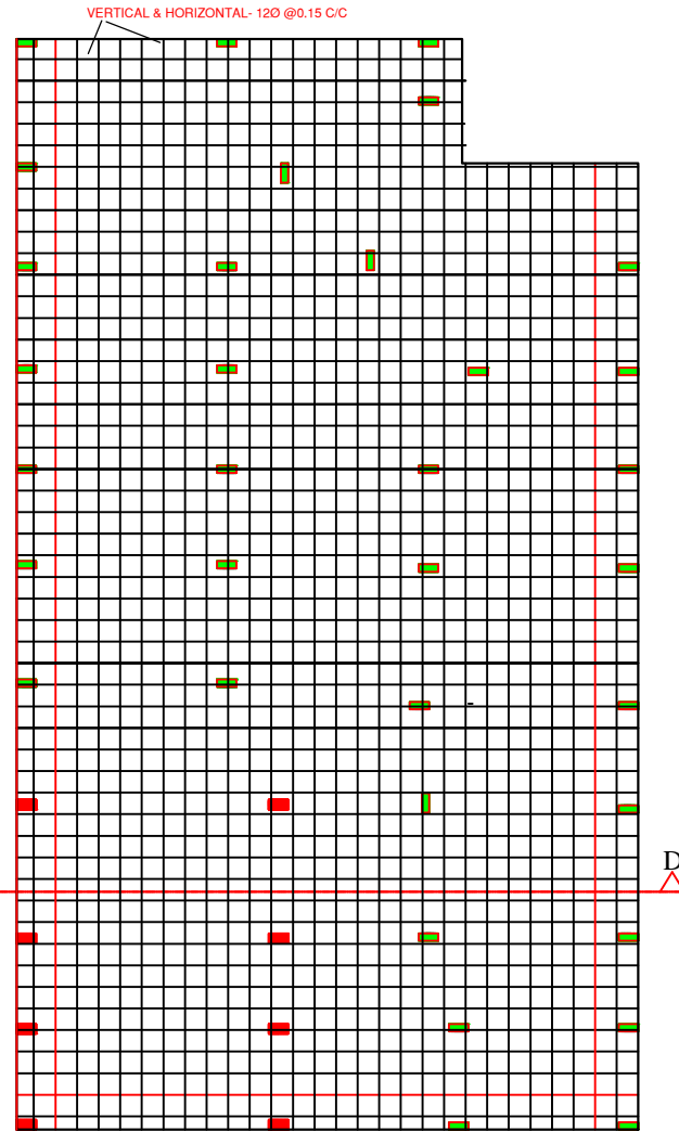
BOTTOM REINFORCEMENT PLAN
