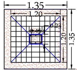
FOUNDATION PLAN
