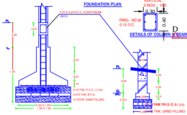
FOUNDATION DETAILS OF COLUMN
