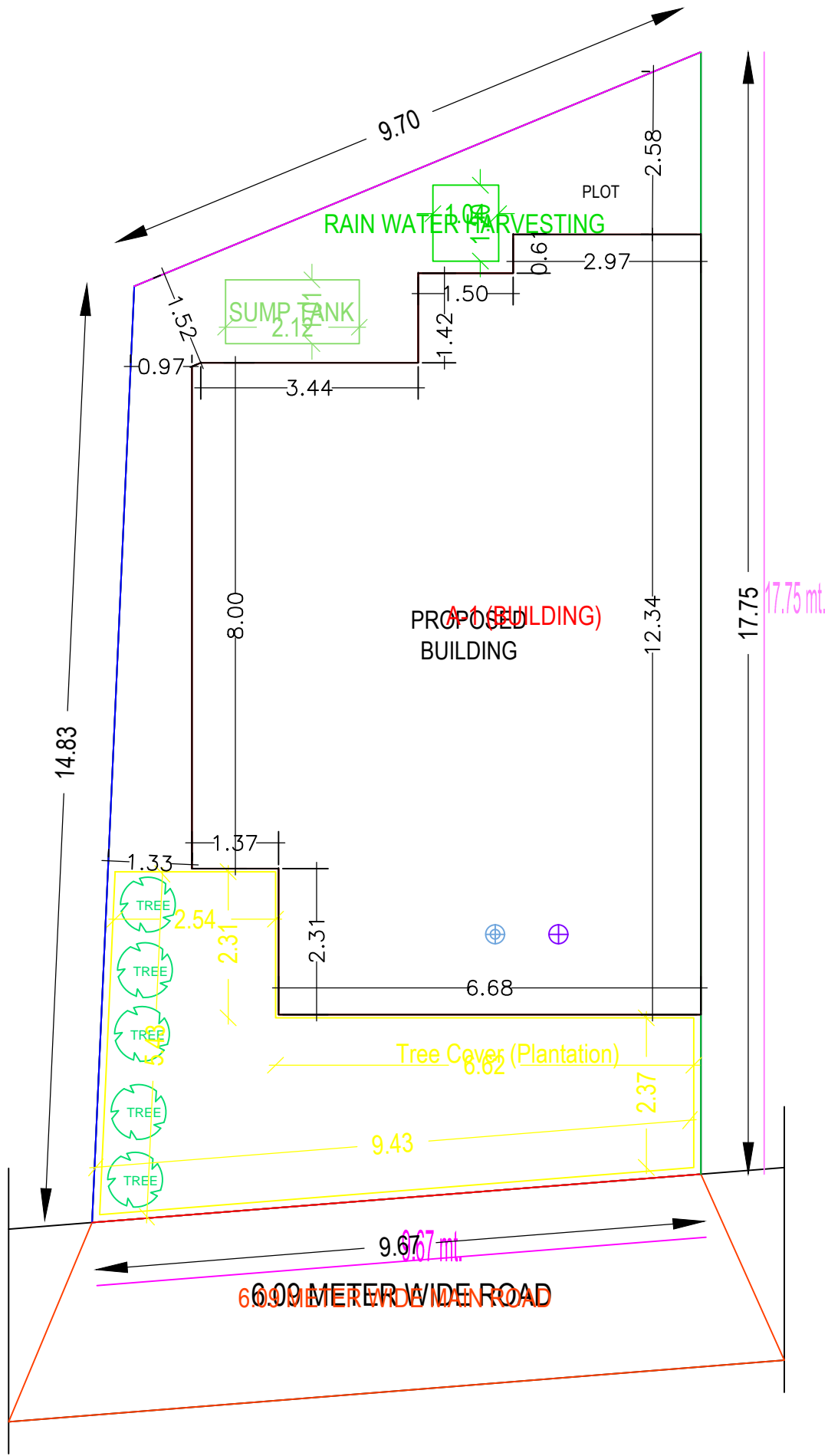
SITE PLAN
