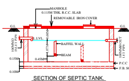
SECTION OF SEPTIC TANK
