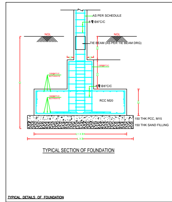
TYPICAL DETAILS OF FOUNDATION
