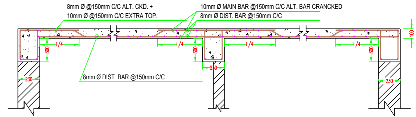
TYPICAL DETAIL OF RCC ROOF SLAB
