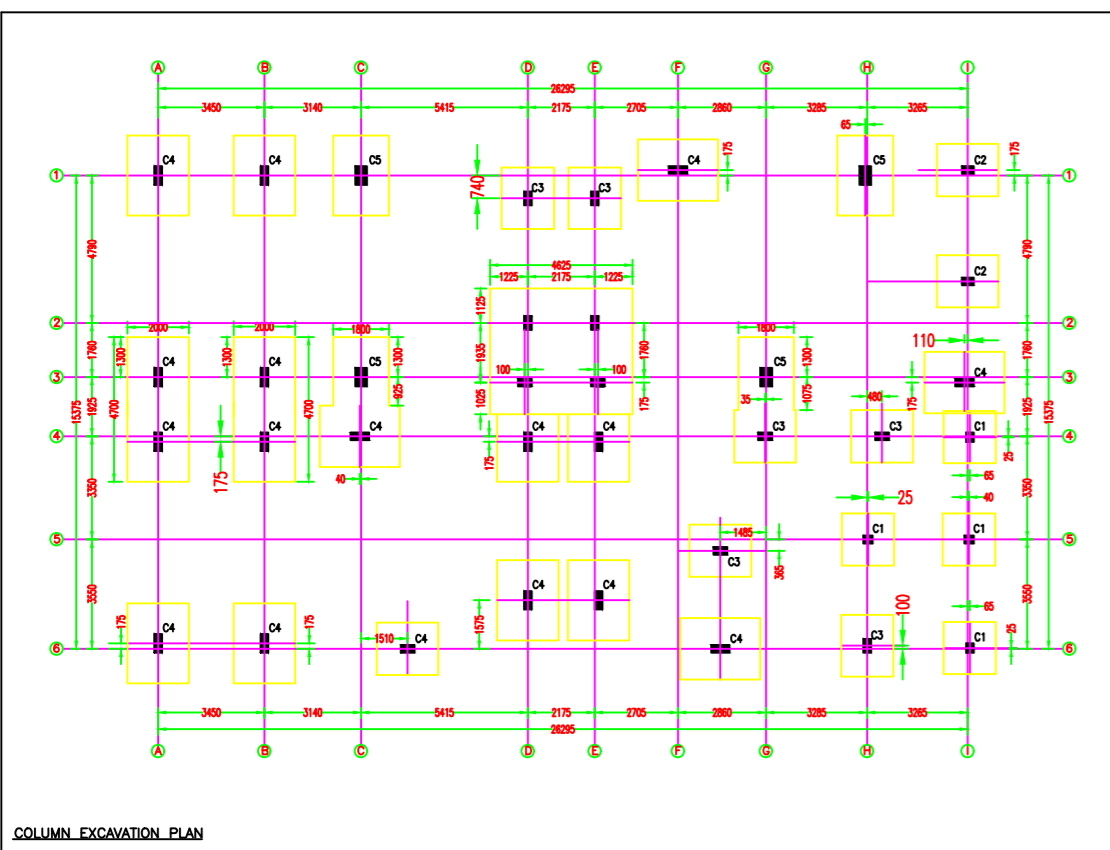
COLUMN EXCAVATION PLAN
