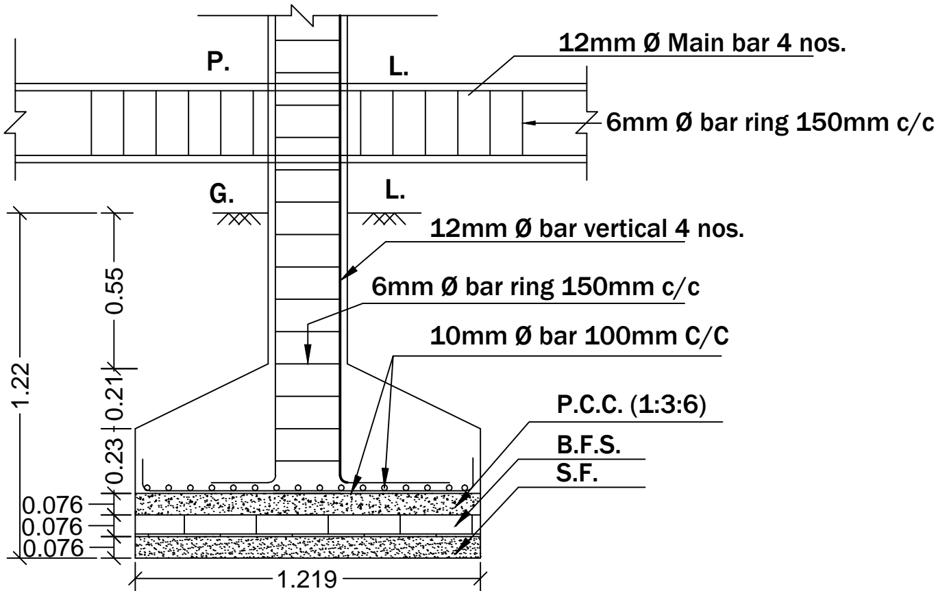
SECTION ON- ZZ
