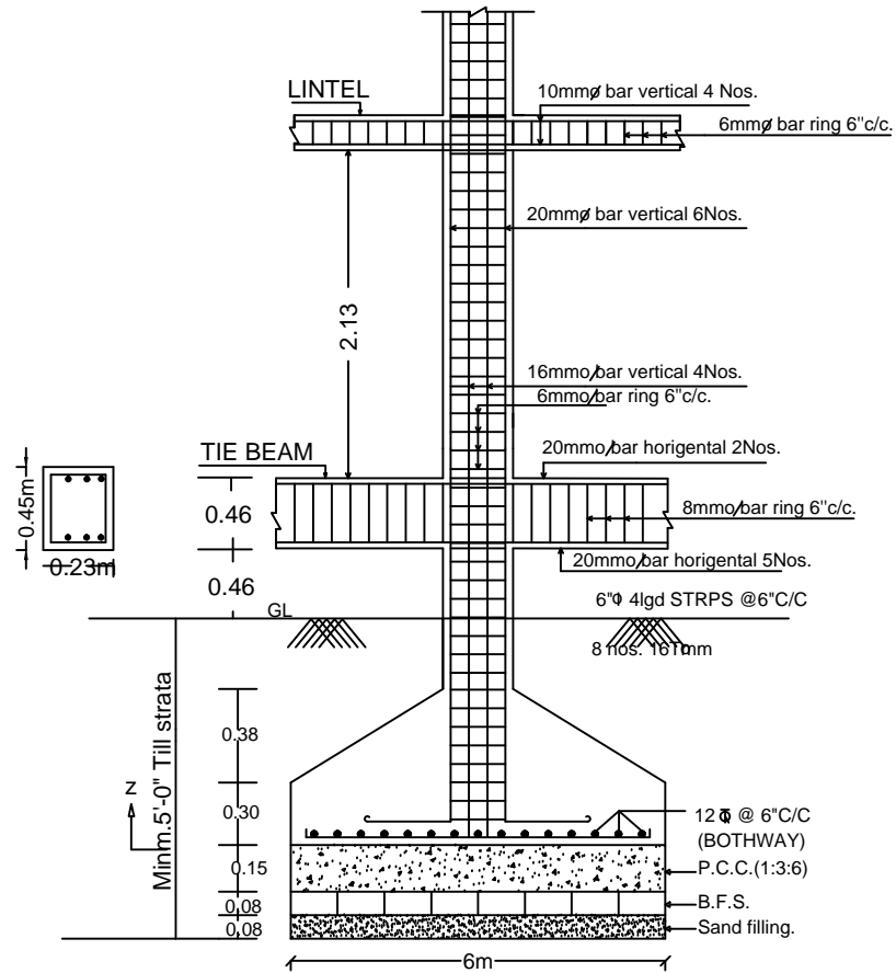
SECTION ON Z-Z
