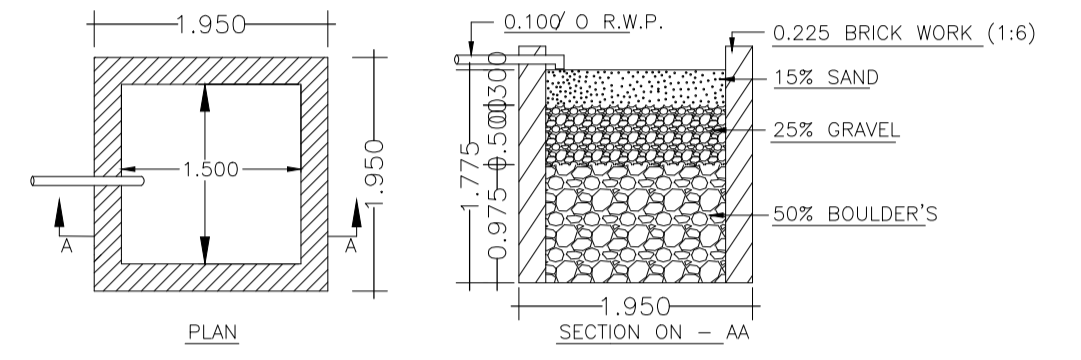
DETAILS OF WATER HARVESTING
