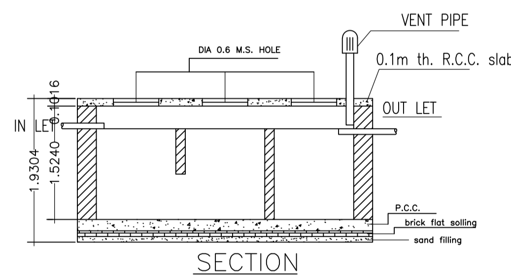
SECTION
