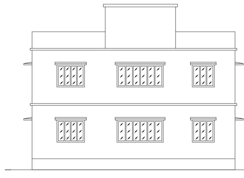
RIGHT SIDE ELEVATION SCALE - 1" = 8'-0"
