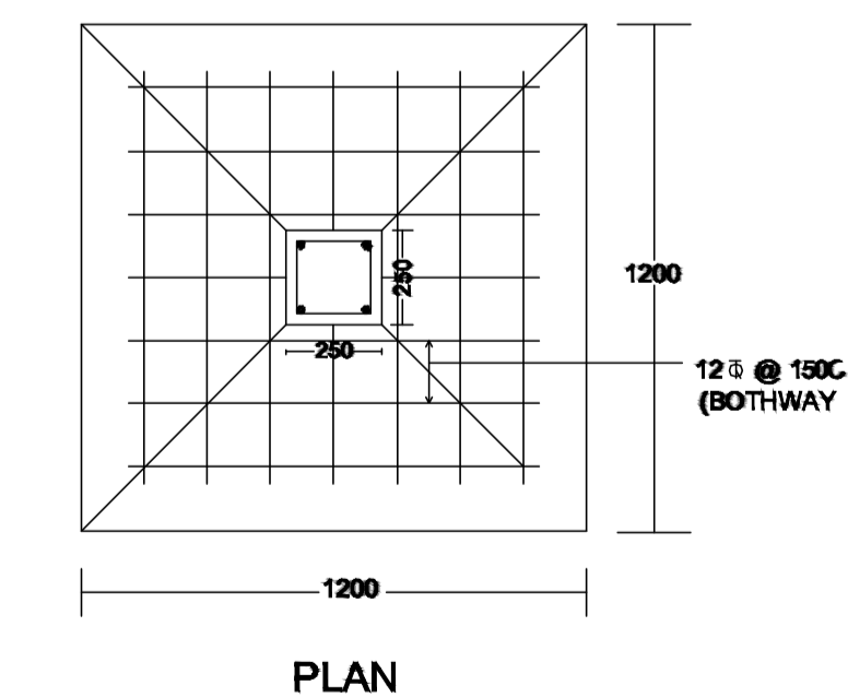
DETAIL OF COLUMNS
