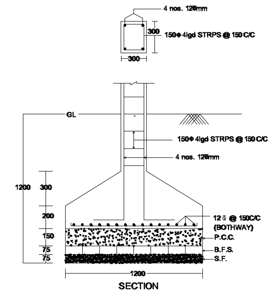
SECTION
