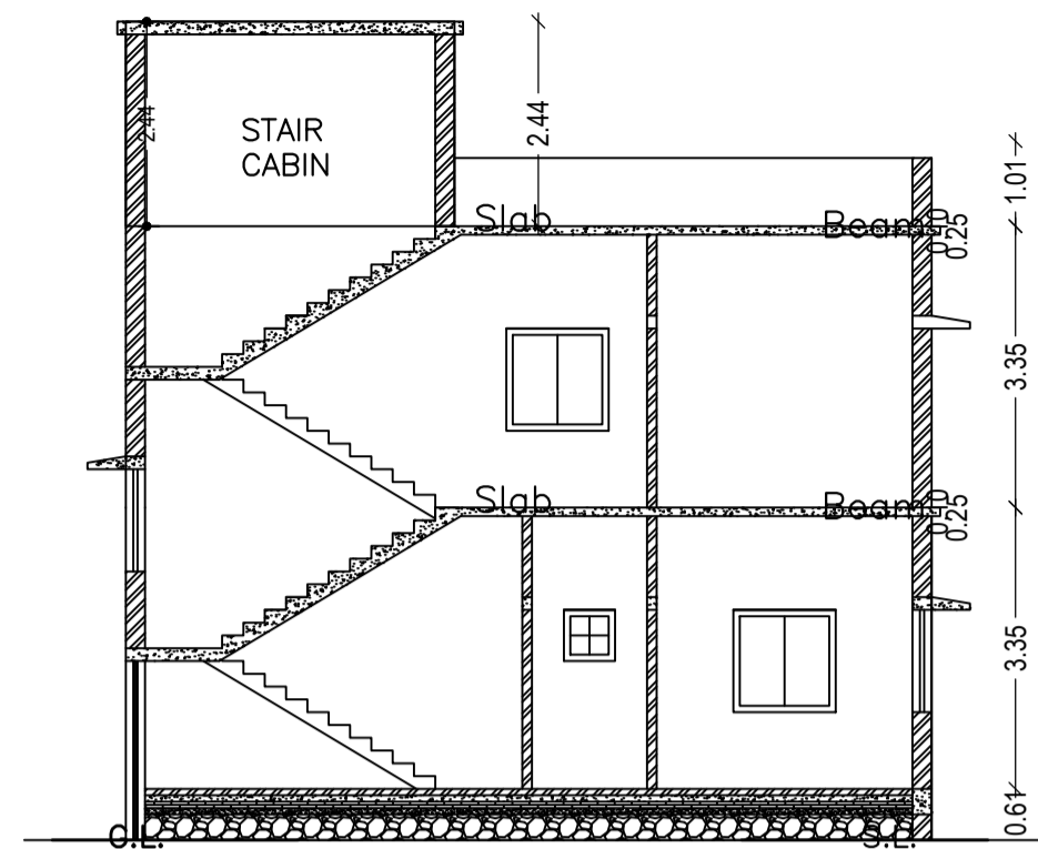
SECTION - XX' SCALE - 1" = 8'-0"
