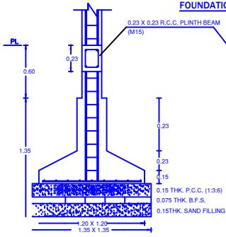
FOUNDATION DETAILS OF COLUMN
