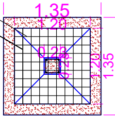
FOUNDATION PLAN
