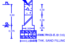
FOUNDATION DETAILS OF WALL
