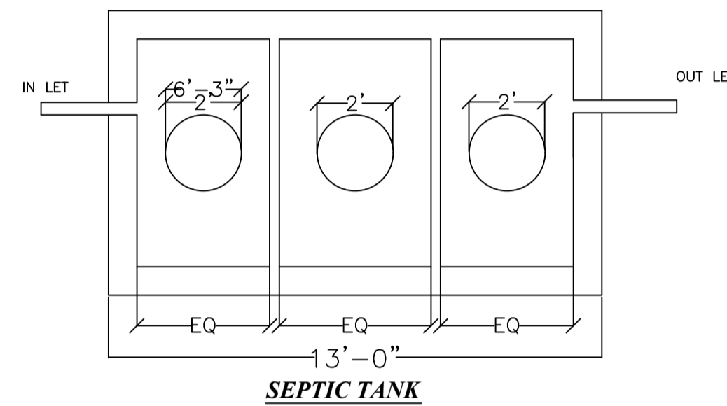
SEPTIC TANK
