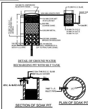
SECTION OF SOAK PIT
