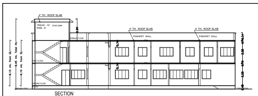
SECTION X-X
