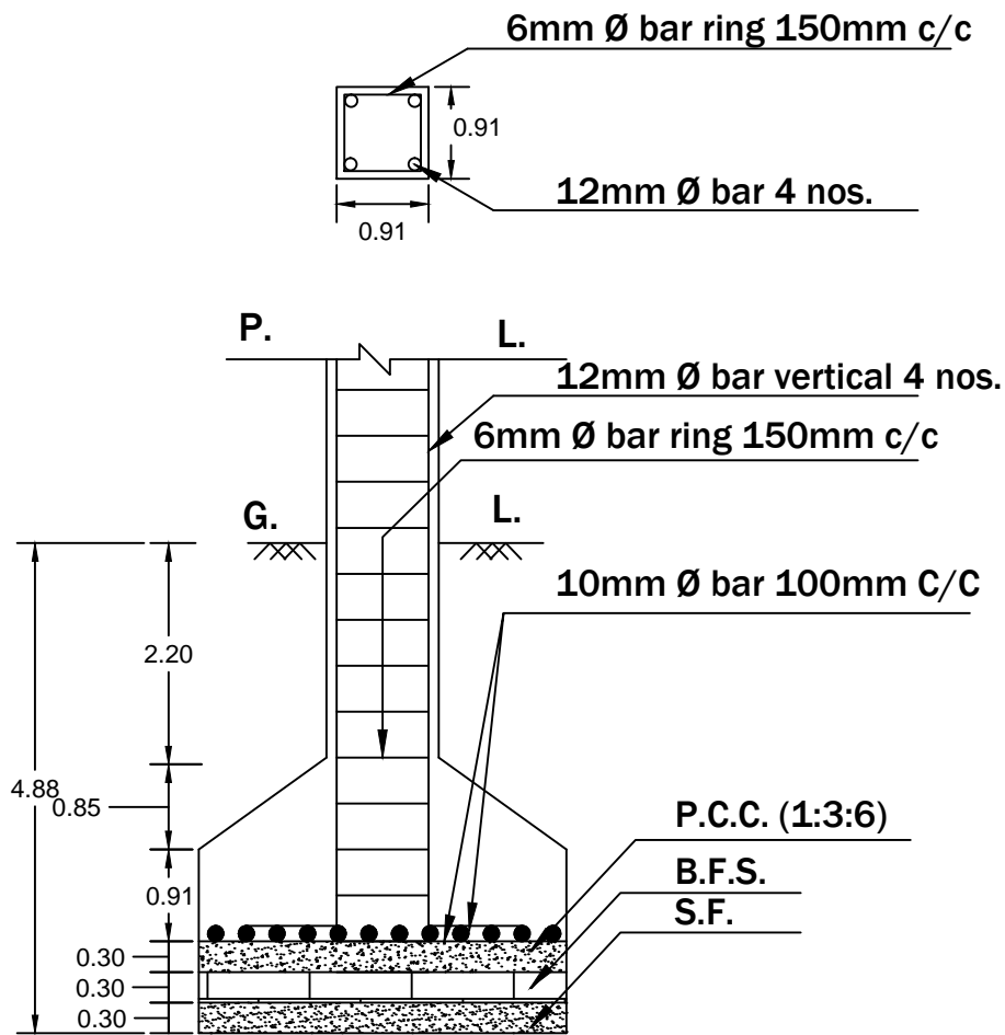
SECTION ON- ZZ SCALE - 1:25
