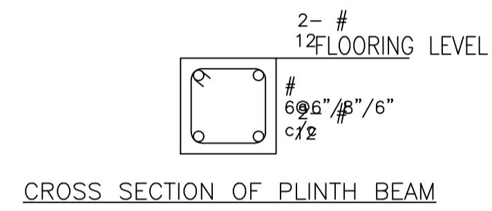
CROSS SECTION OF PLINTH BEAM
