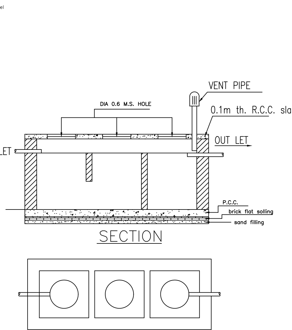
DETAILS OF SEPTIC TANK
