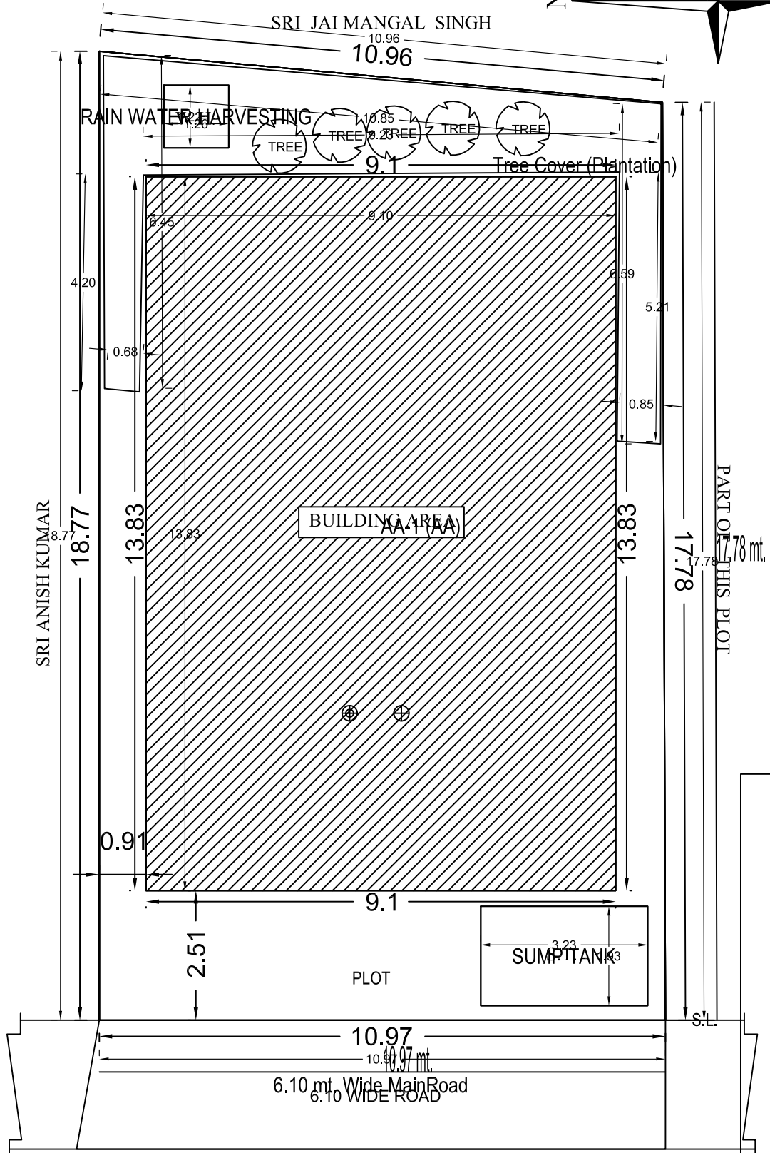
SITE PLAN SITE PLAN
