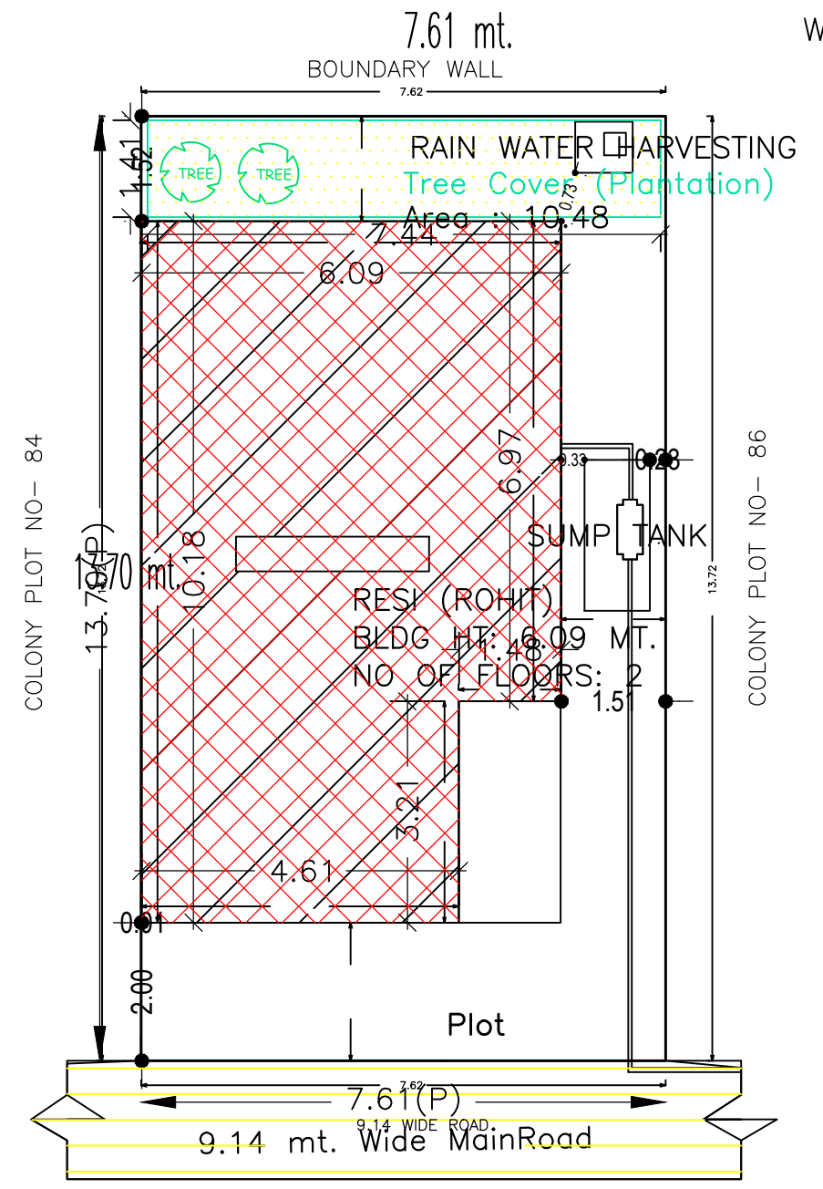
SITE PLAN SCALE :- 1IN=200
