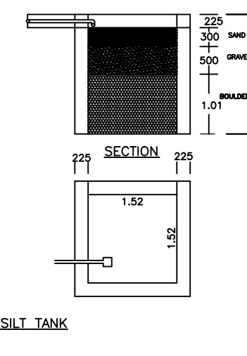
PLAN OF RAIN WATER HARVESTING (SCALE:- 1:25)
