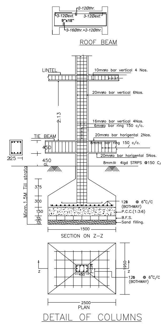
DETAIL OF COLUMNS SCALE:- 1:25
