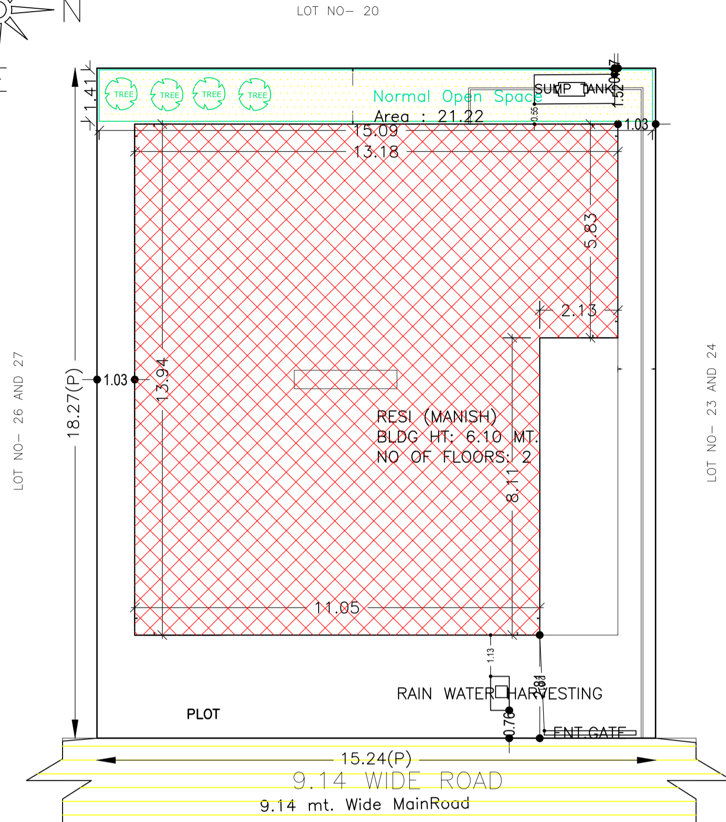
SITE PLAN SCALE :-1IN=200 SITE PLAN
