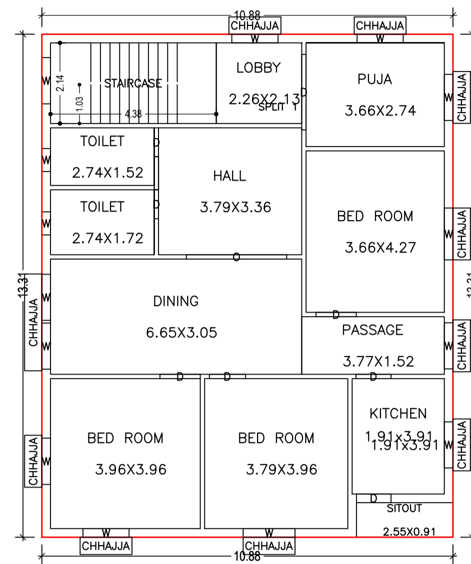
TYPICAL - FIRST & SECOND FLOOR PLAN (Proposed) (SCALE 1:100)
