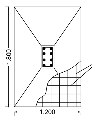
COLUMN DETAILS SCALE:- 1:50
