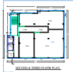
SECOND & THIRD FLOOR PLAN
