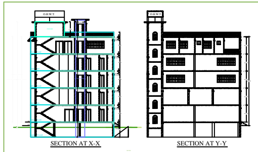
SECTION AT X-X
