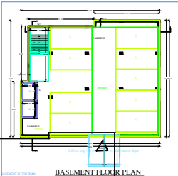
BASEMENT FLOOR PLAN
