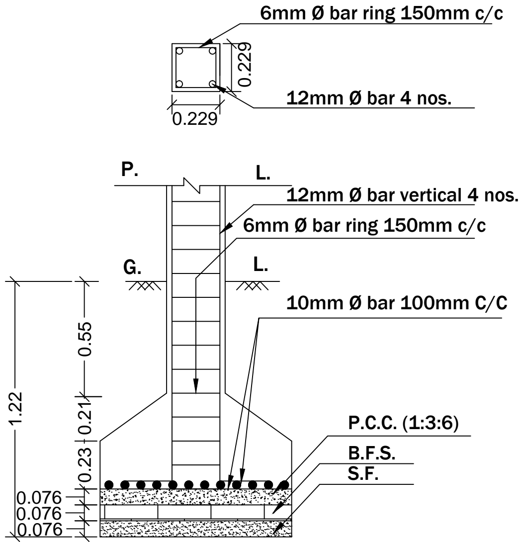
SECTION ON- ZZ SCALE - 1:25
