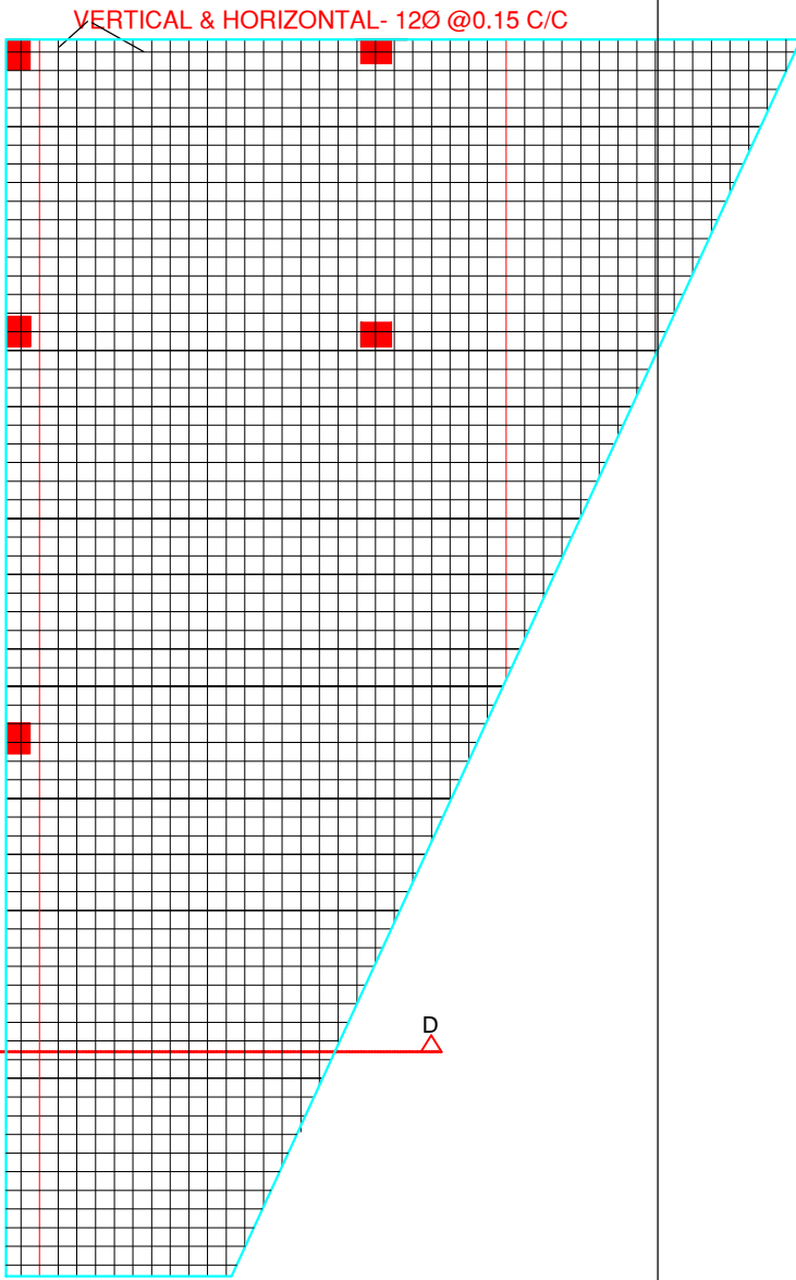
BOTTOM REINFORCEMENT PLAN
