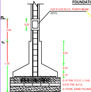
FOUNDATION DETAILS OF COLUMN
