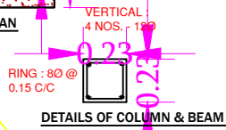
DETAILS OF COLUMN & BEAM
