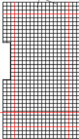
BOTTOM REINFORCEMENT PLAN
