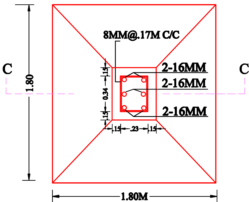
R.C.C. COL. FDN. PLAN SCALE -1:25
